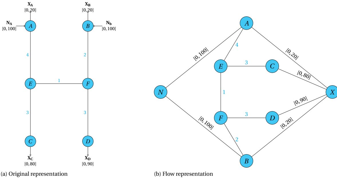
Figure 3.11: Advanced H-network
