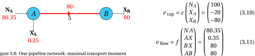
Figure 3.8: One pipeline network: maximal transport moment
