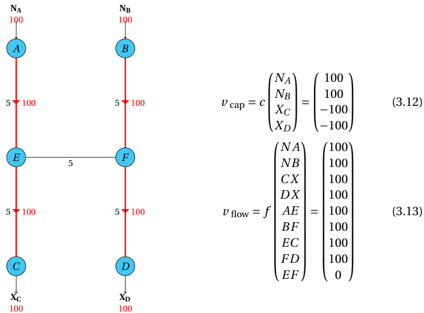
Figure 3.10: Simple H-network: maximal transport moment
