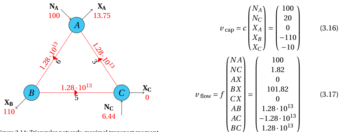
Figure 3.14: Triangular network: maximal transport moment
