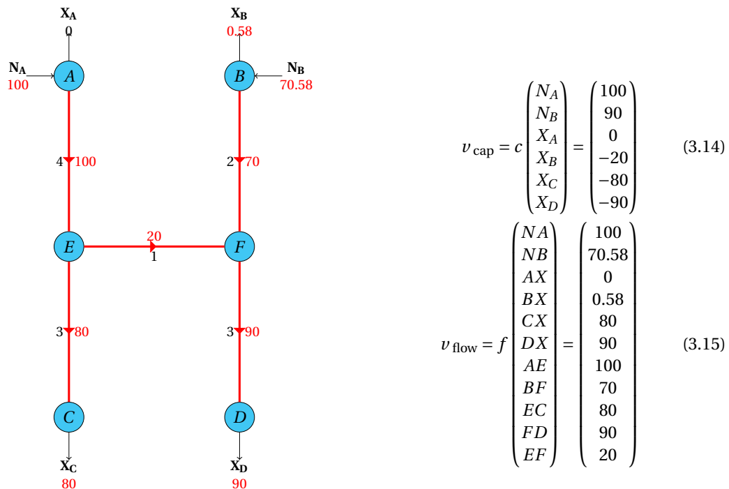
Figure 3.12: Advanced H-network: maximal transport moment
